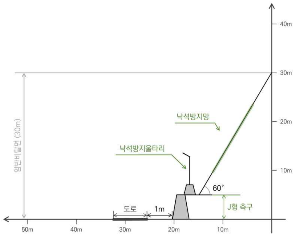
[횡단면도]
